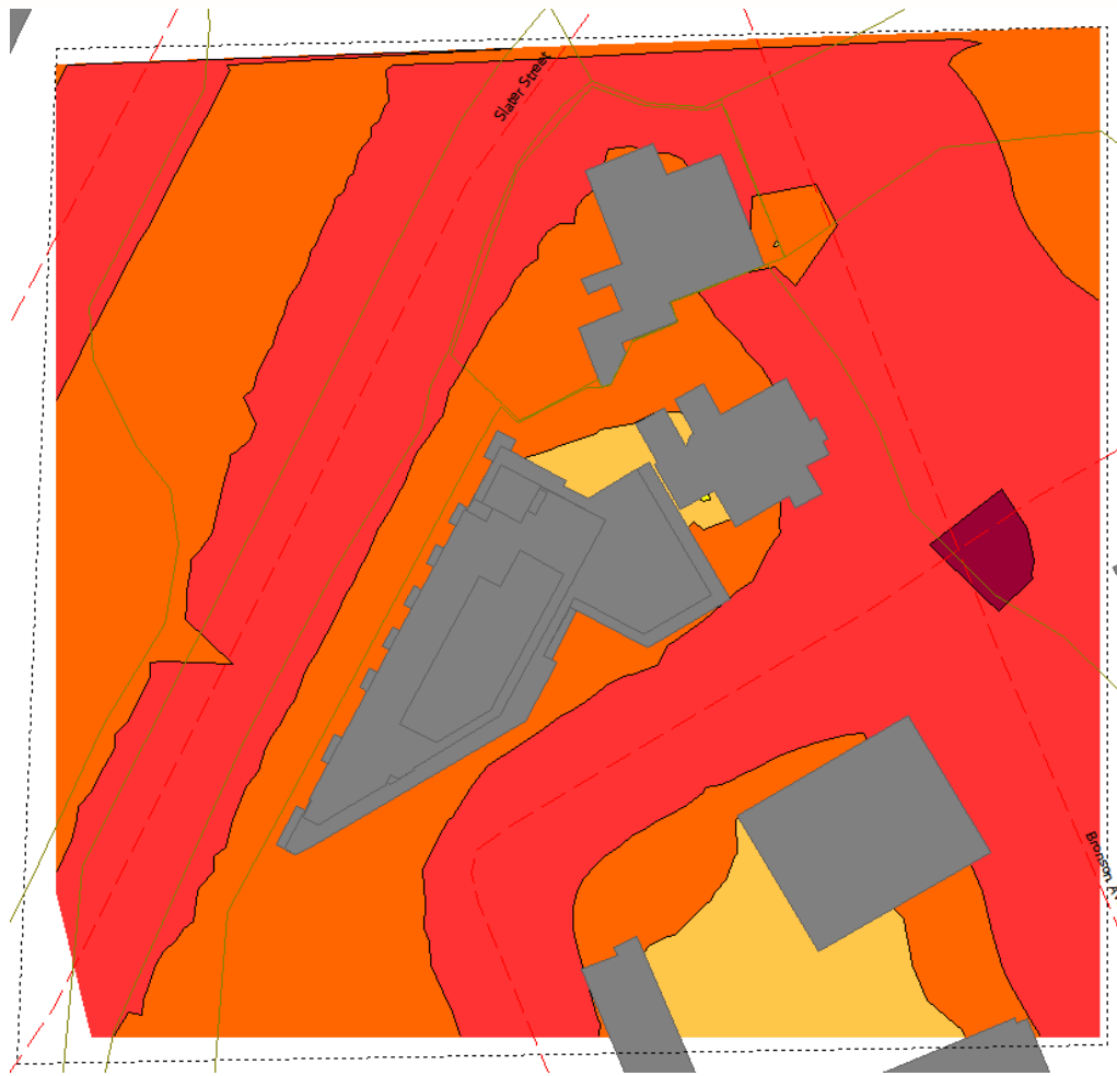
FIGURE 6: NIGHTTIME TRANSPORTATION NOISE CONTOURS (4.5 M ABOVE GRADE)
