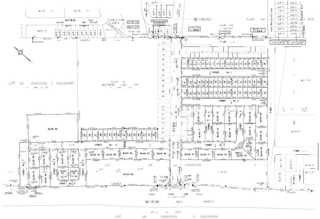
Figure 16. Draft Plan of Subdivision - Phases 4A and 4B.
