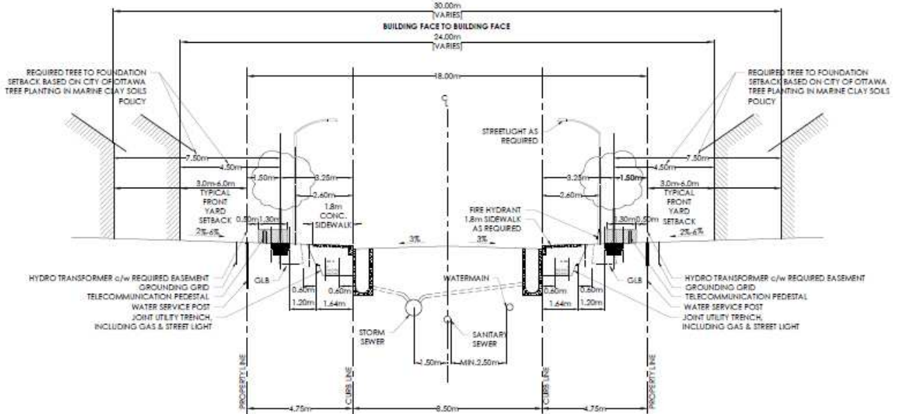
Figure 18. Typical 18m cross section
