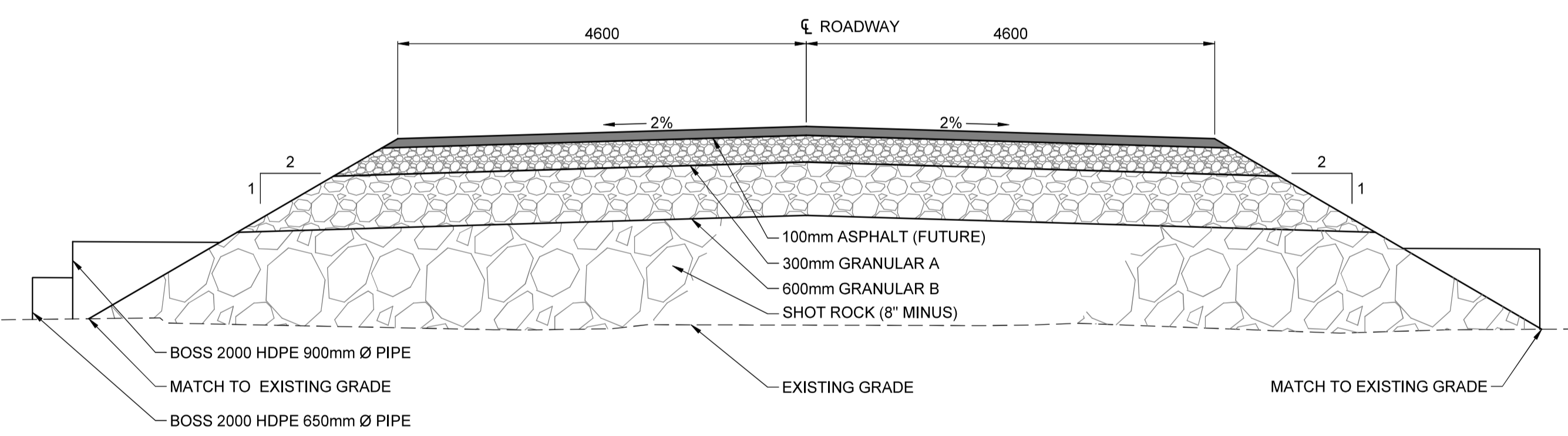
TYPICAL ROADWAY SECTION SCALE: 1:50
