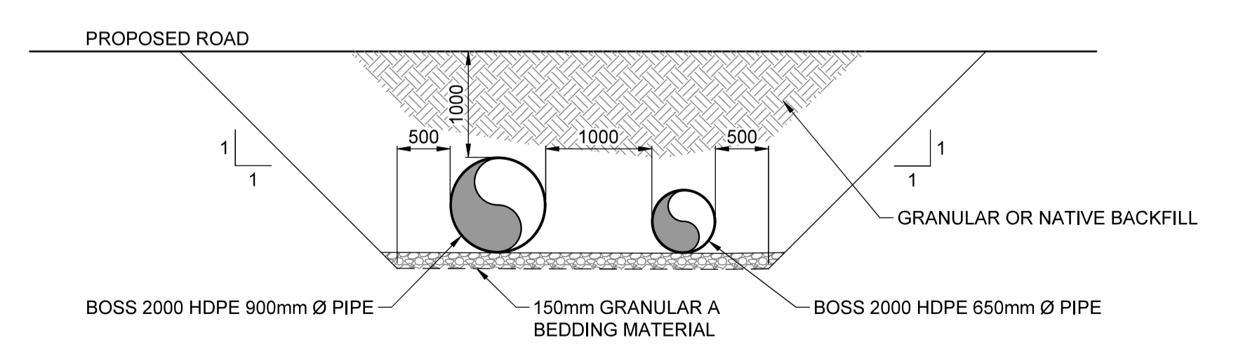
TYPICAL CULVERT CROSS SECTION AND BACKFILL SCALE: 1:50
