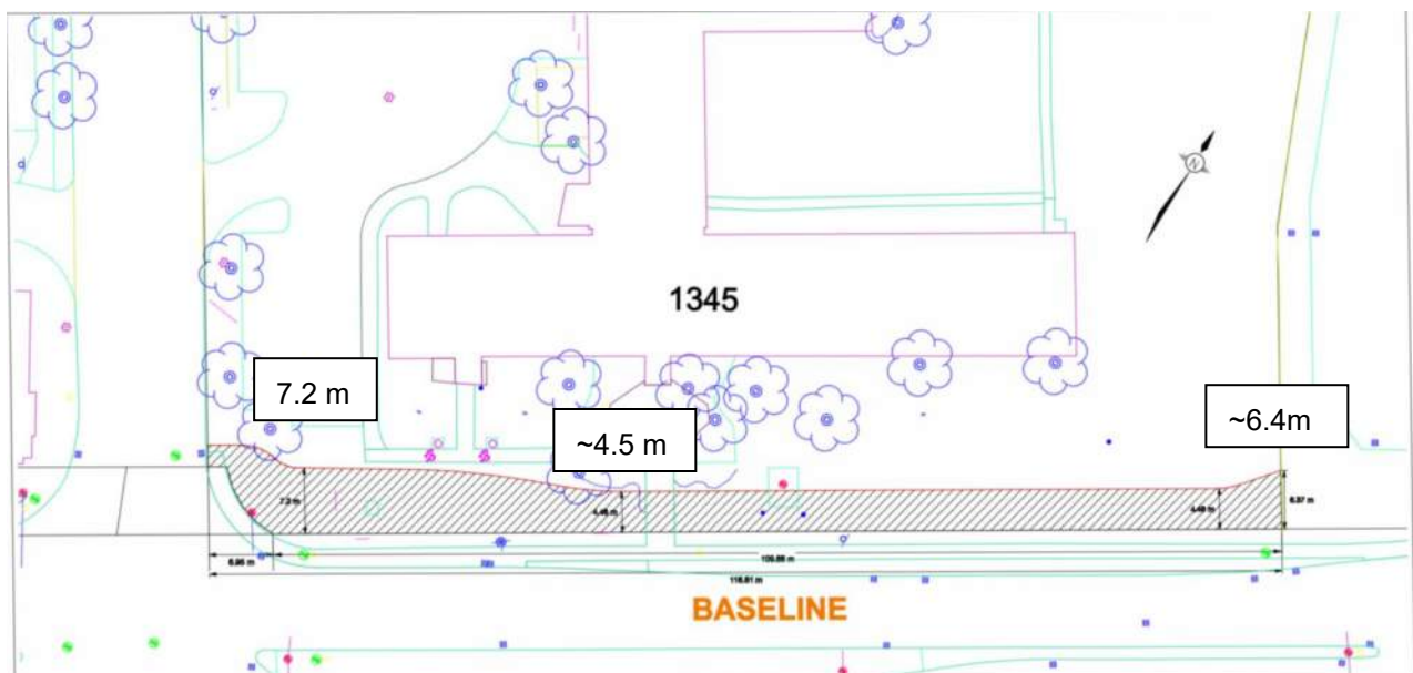
Figure 15. Baseline Road Transitway ROW requirements.
