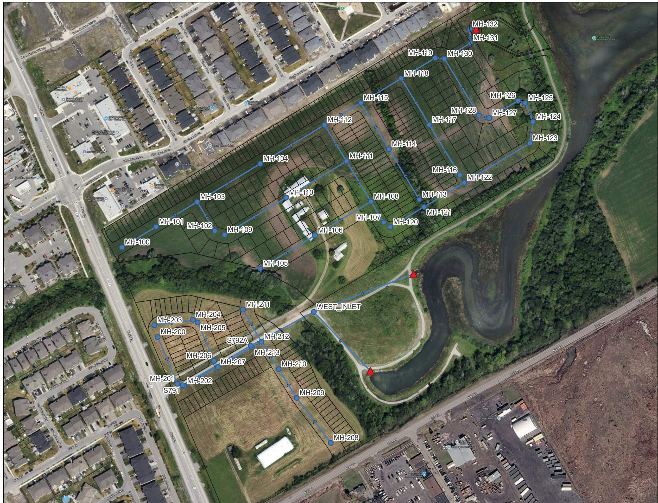
Figure A1 - Storm Sewer Plan
