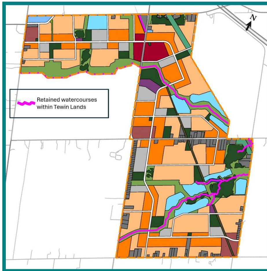
Figure 53: Retained Existing Watercourses
