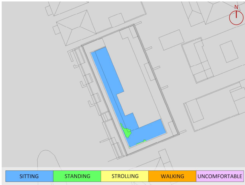
FIGURE 8B: SUMMER – WIND COMFORT, AMENITY TERRACE
