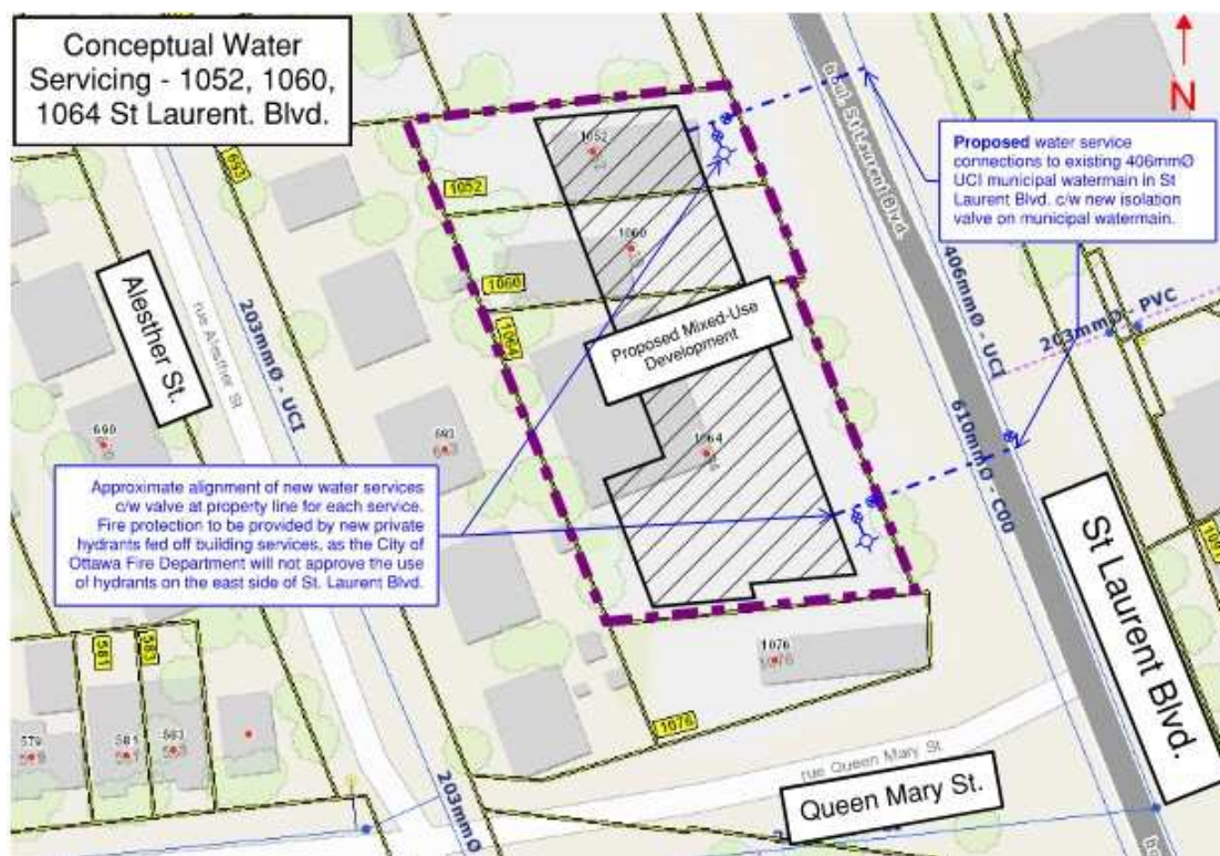
Figure 3: Conceptual Water Servicing Layout
