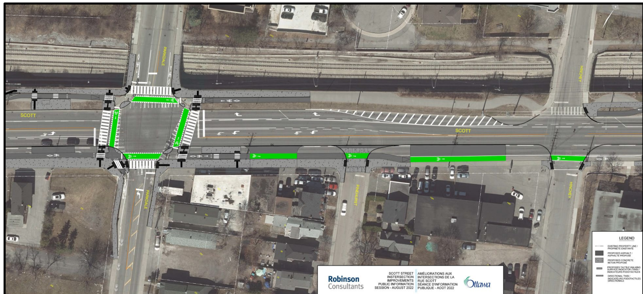
Figure 14: Scott St Improvements – Protected Intersection
