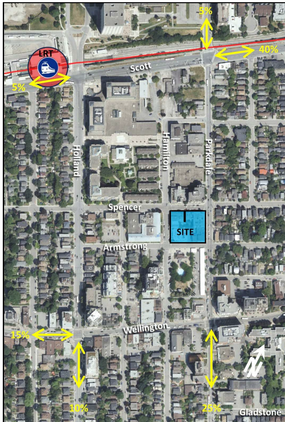
Figure 18: Site Generated Vehicle Traffic Percent Distribution
