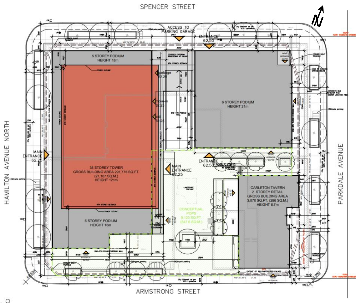
Figure 2: Proposed Site Plan – Ground Floor Plan (1 May 2026)
