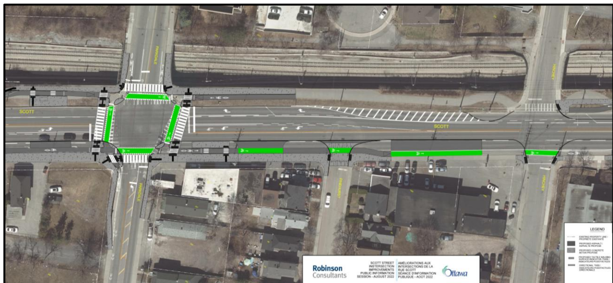
Figure 14: Scott St Improvements – Protected Intersection
