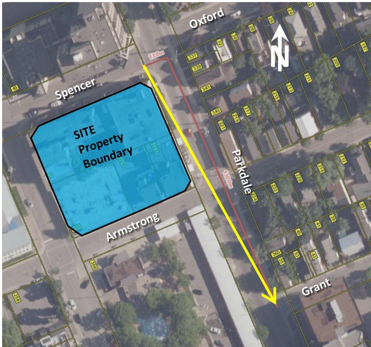
Figure 10: Sightline Analysis, Eastbound Left Turn from Spencer Street
