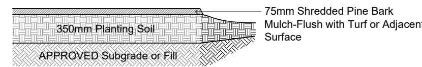
PLANTING BED - TYPICAL NTS
