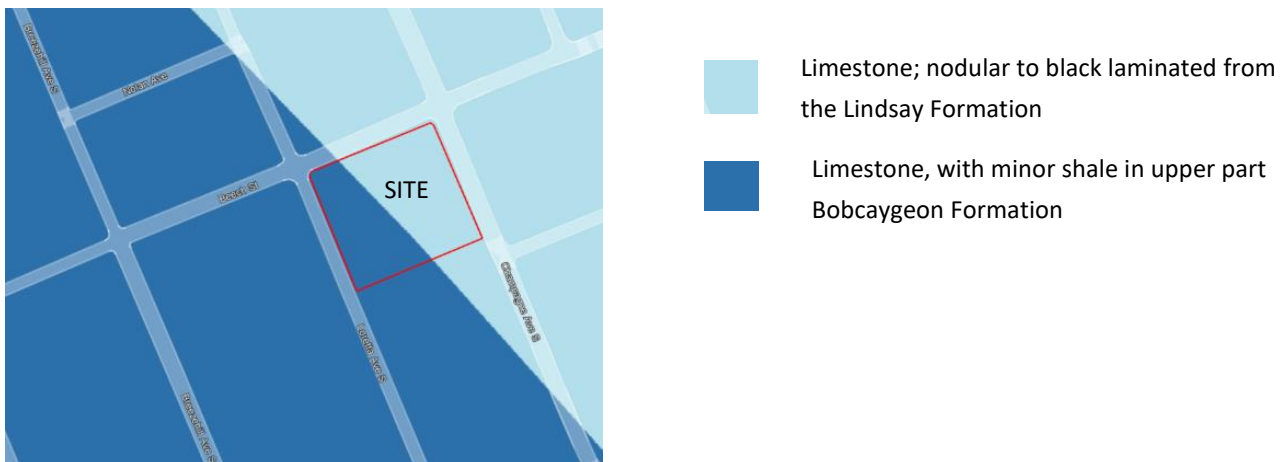
Image 2 – Bedrock Geology
