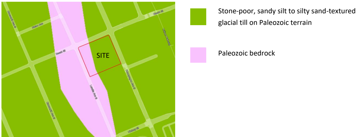
Image 1 – Surficial Geology
