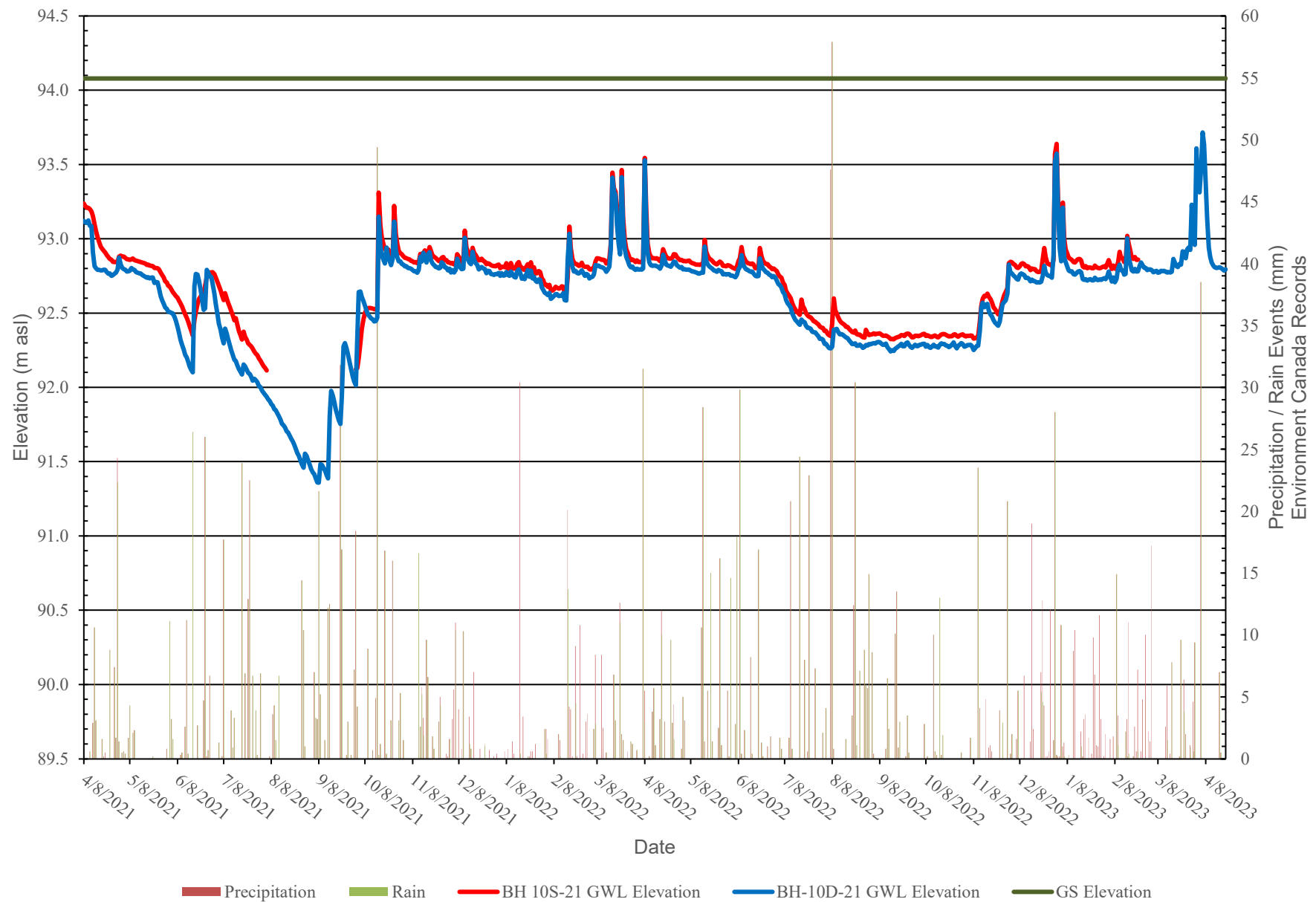
Figure 10: BH 10-21 - Groundwater Monitoring Levels vs Precipitation Data
