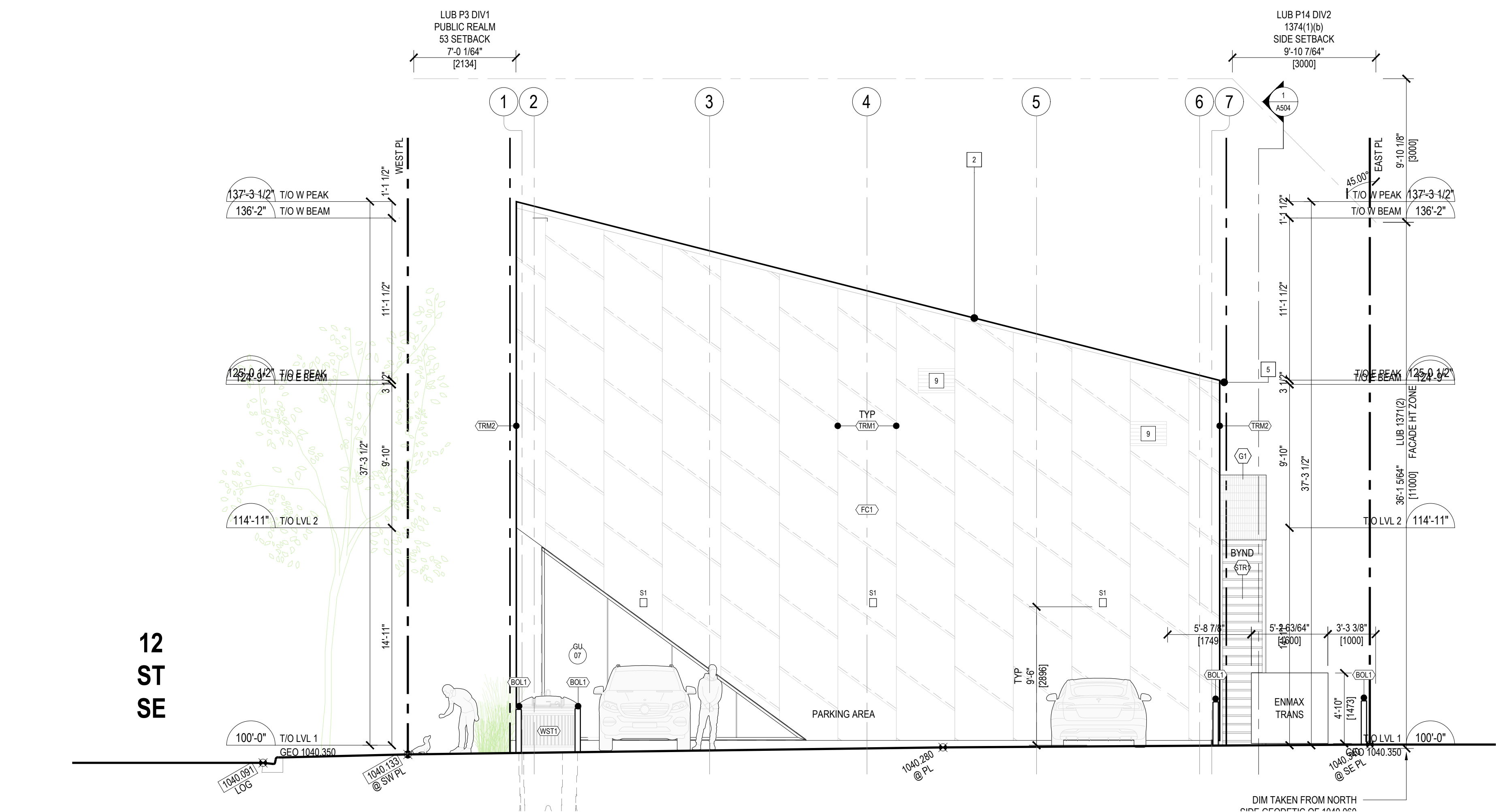
2 SOUTH BLDG ELEV A301 3/16" = 1'-0"
