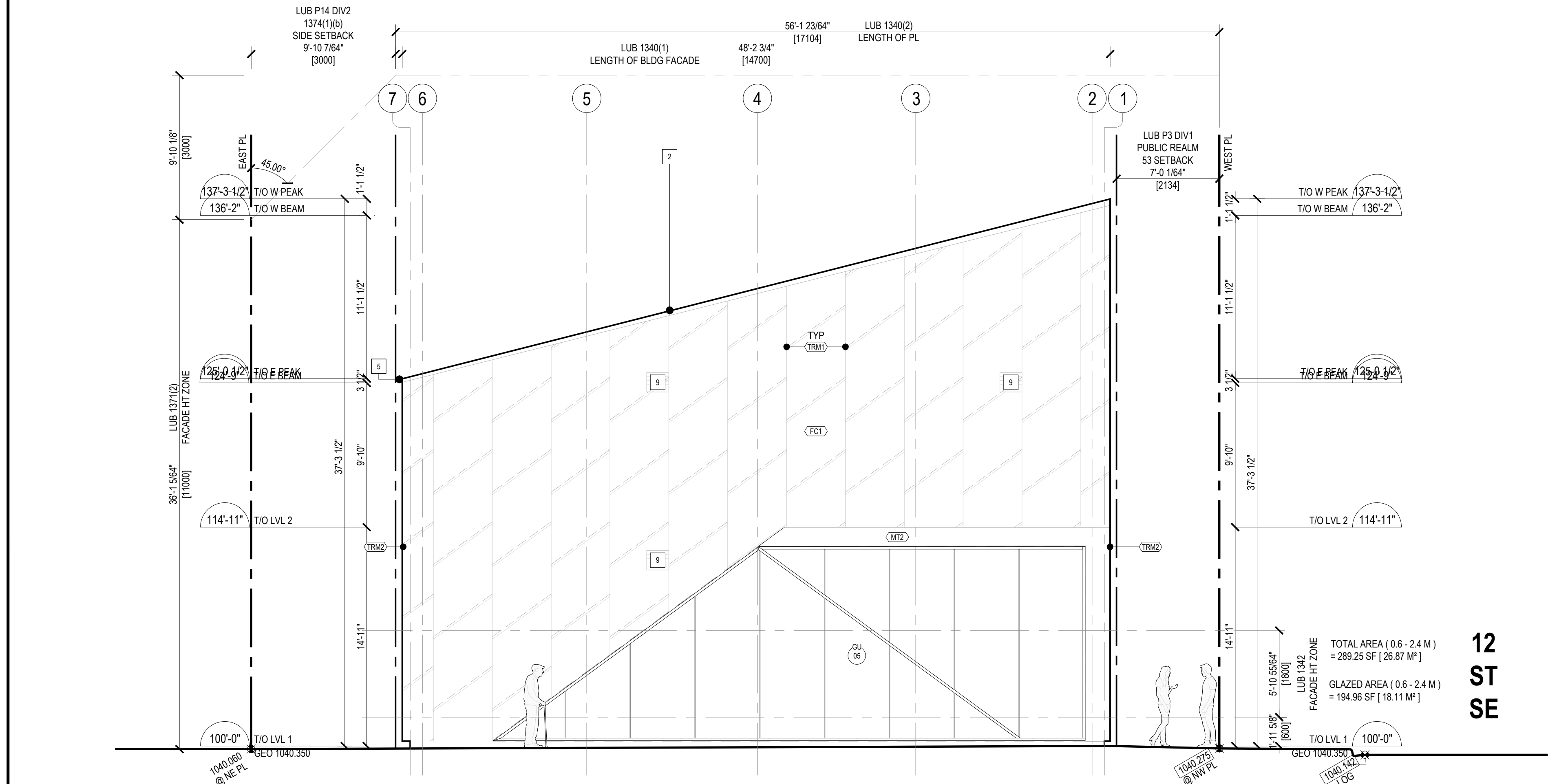
2 NORTH BLDG ELEV 1:75
