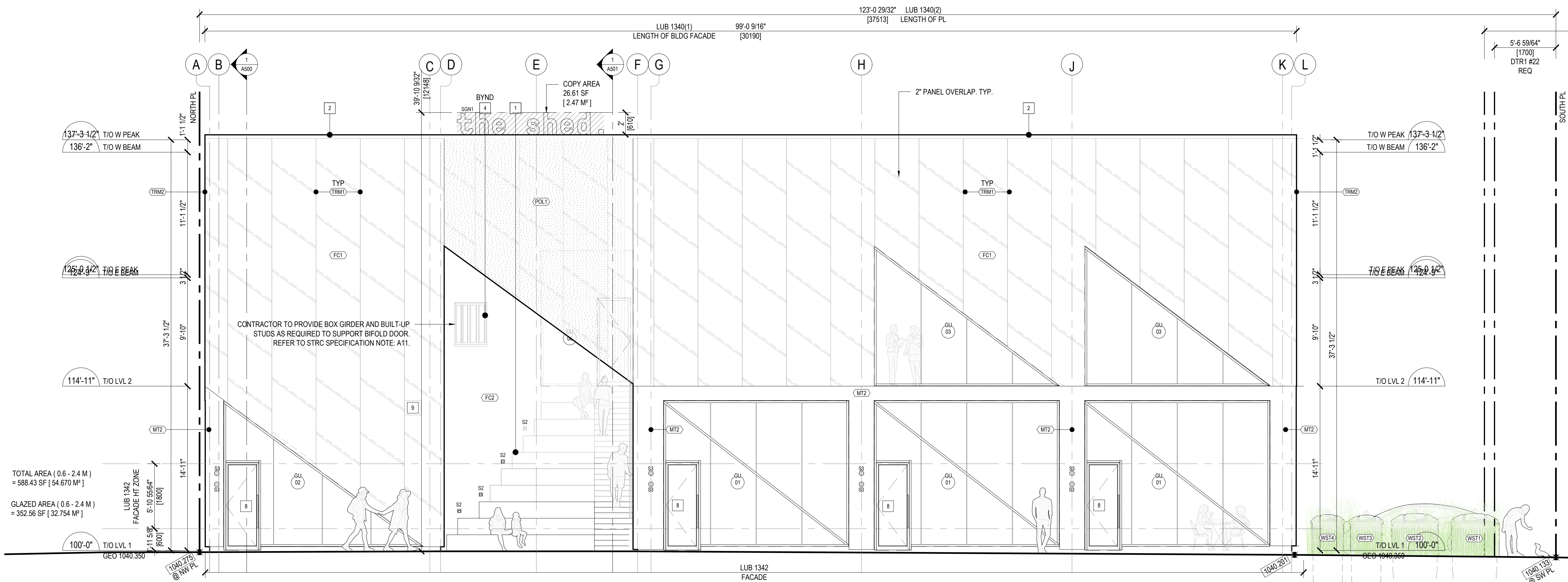
1 WEST BLDG ELEV A301 3/16" = 1'-0"
