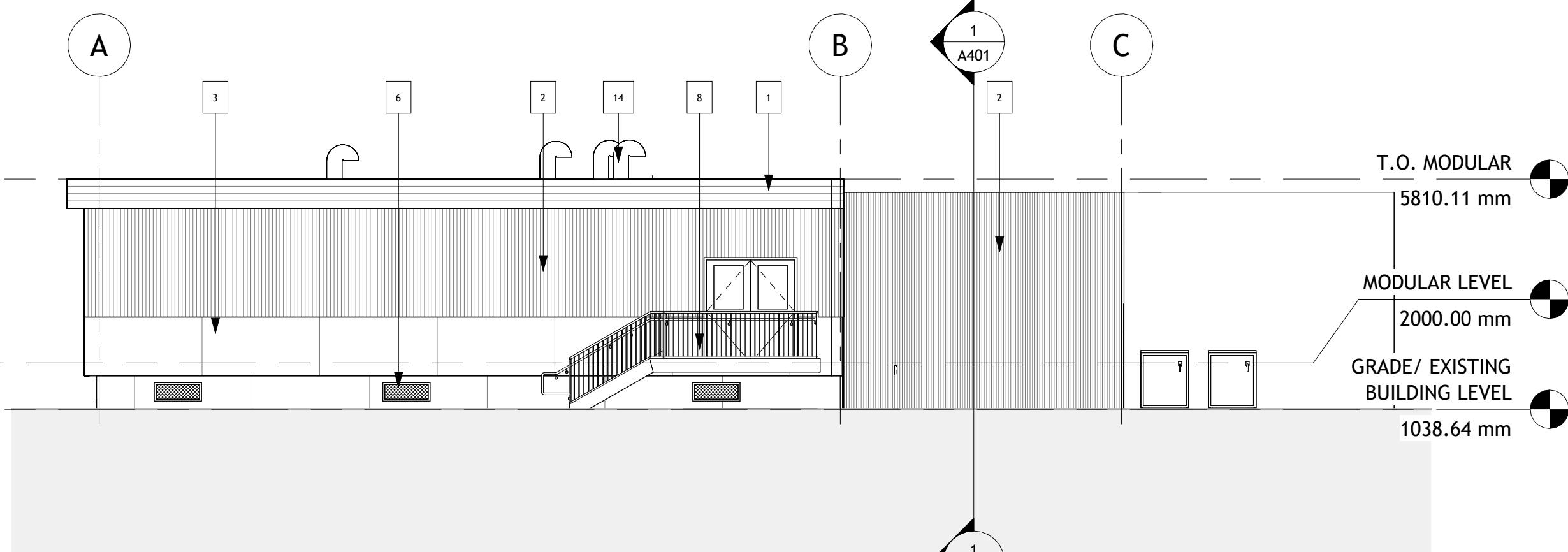
4 WEST ELEVATION 1 : 100
