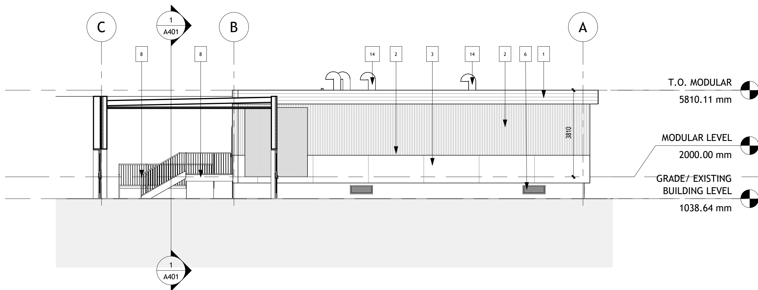
1 EAST ELEVATION 1 : 100
