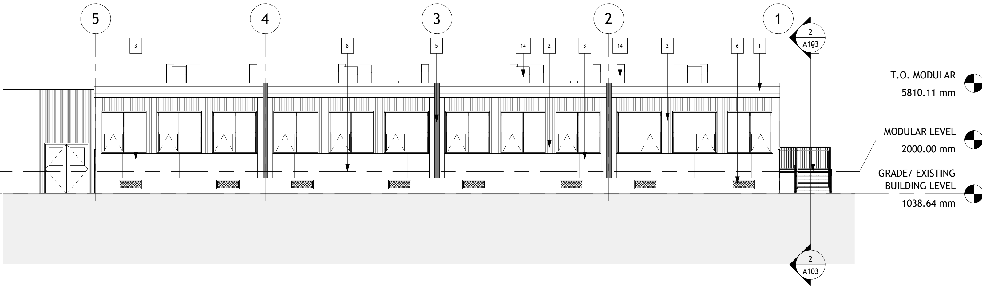
2 NORTH ELEVATION 1 : 100
