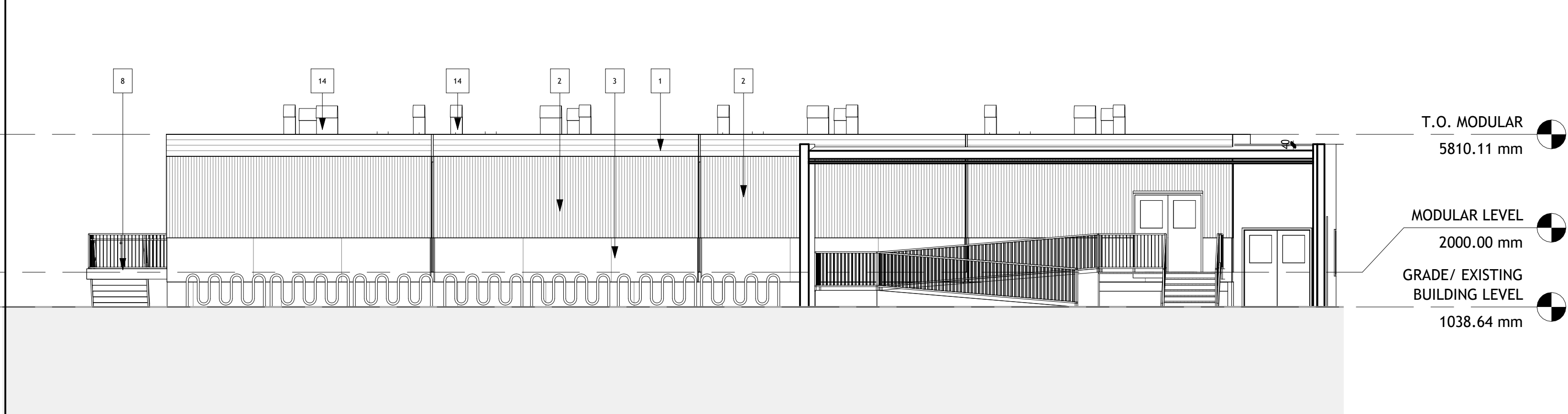
3 SOUTH ELEVATION 1 : 100
