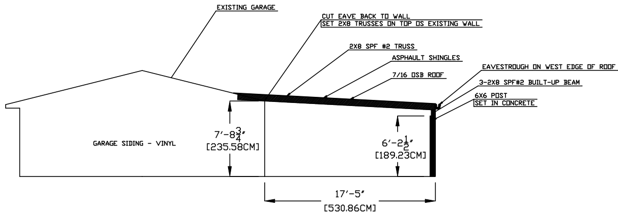
FRONT VIEW 343 MANDRA DRIVE NE
