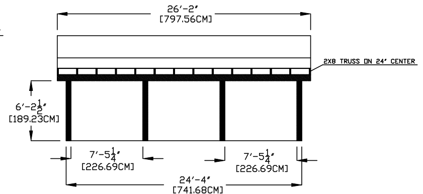
SIDE VIEW 343 MANDRA DRIVE NE
