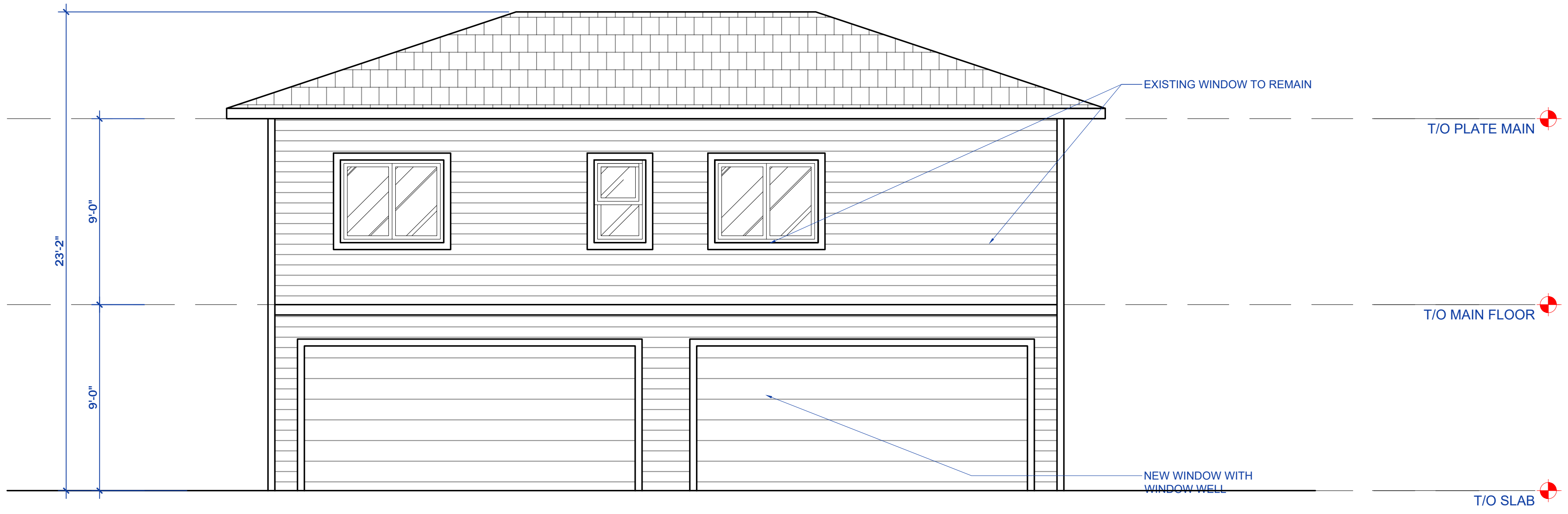
1 D5 GARAGE SUITE SOUTH (REAR) ELEVATION SCALE: 1/4"=1' -0"
