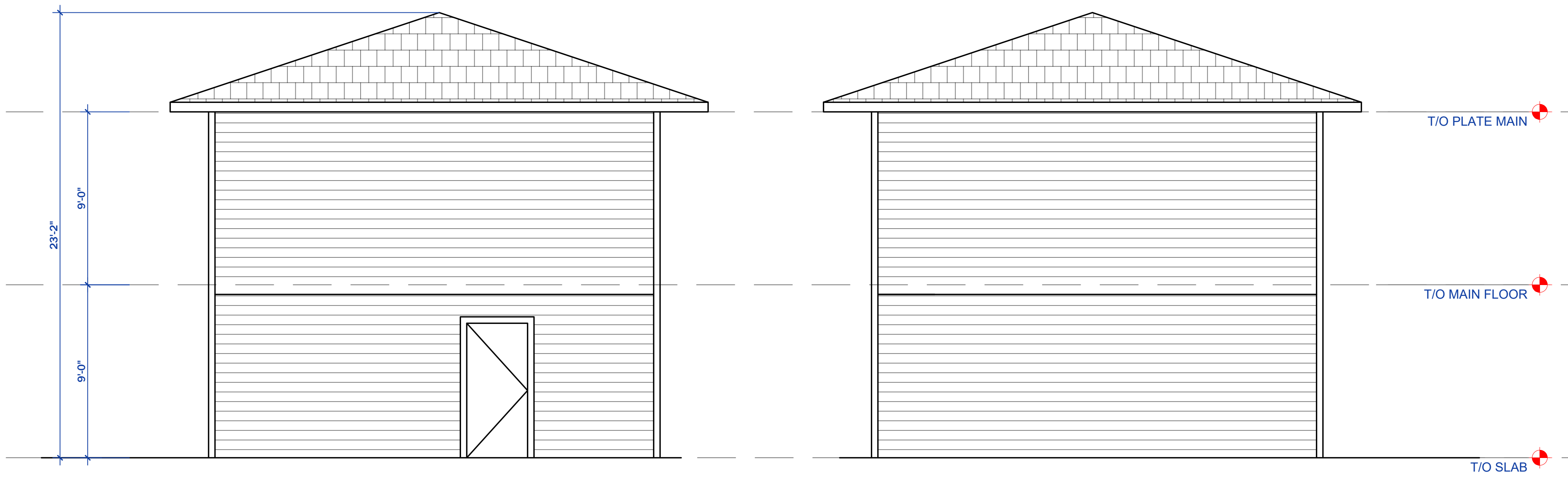
2 D5 GARAGE SUITE EAST (LEFT) ELEVATION SCALE: 1/4"=1' -0"
