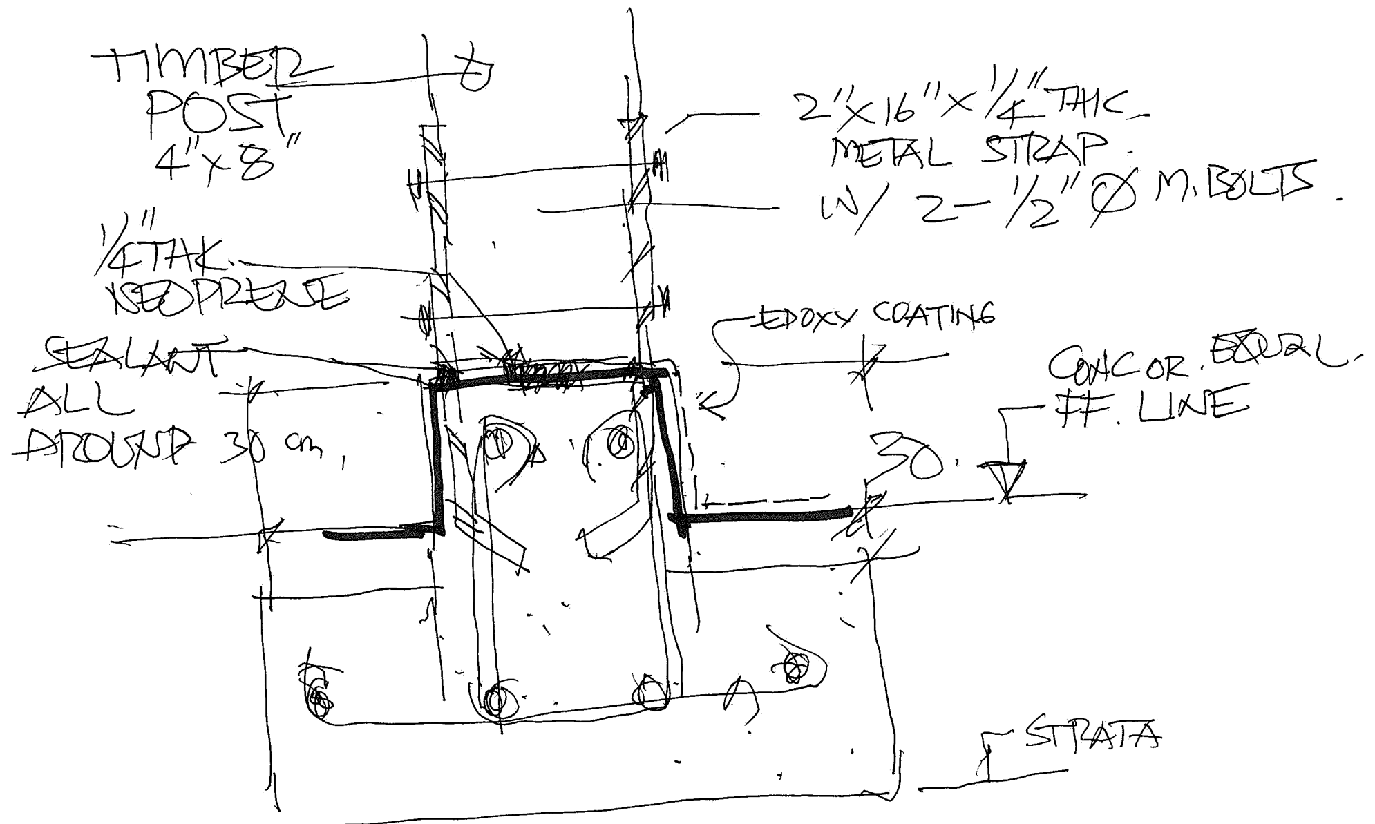
TYPICAL STRAP DET. TO - TIMBER POST.
