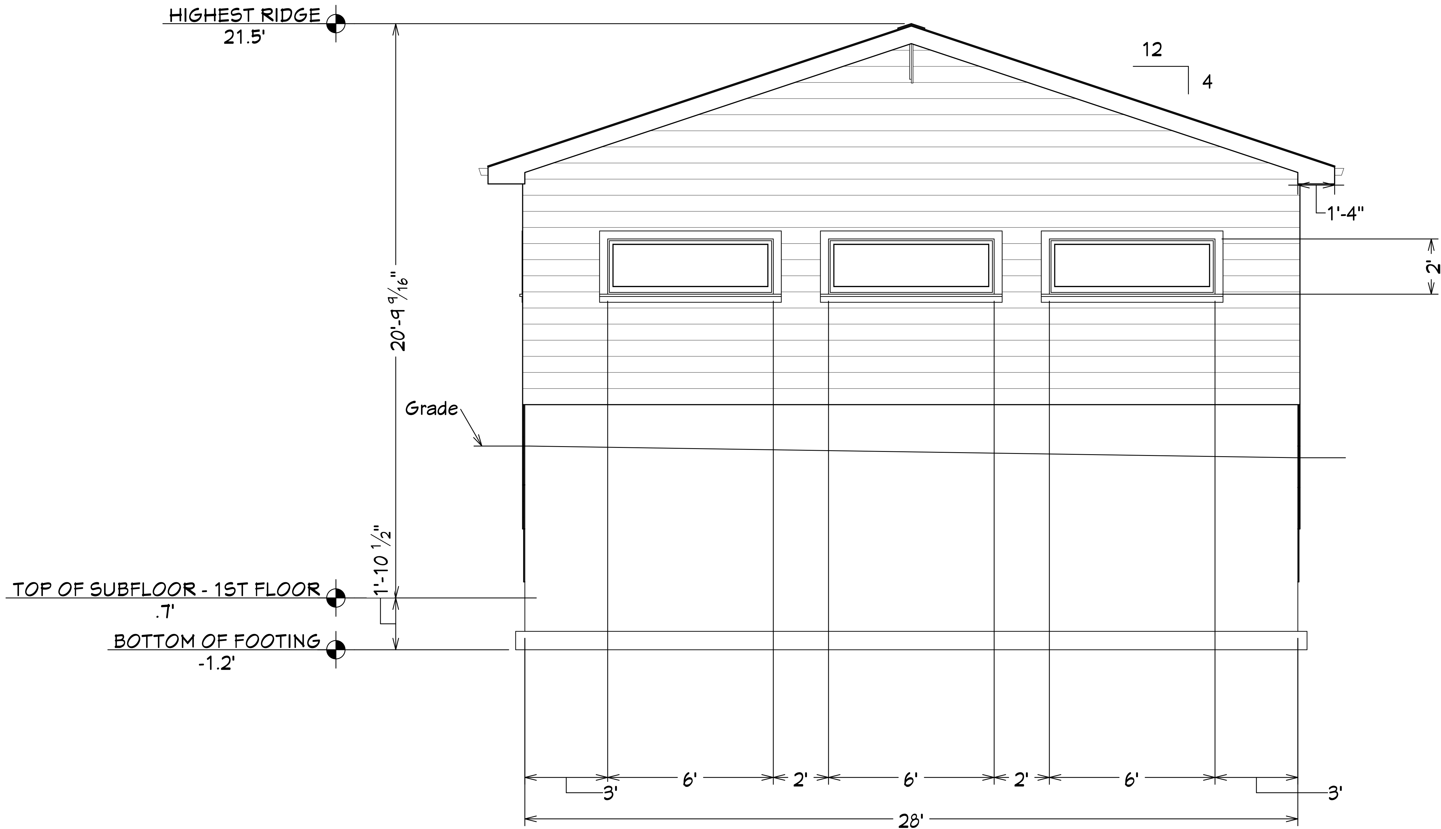
E9 EXTERIOR ELEVATION REAR 1/2 IN = 1 FT
