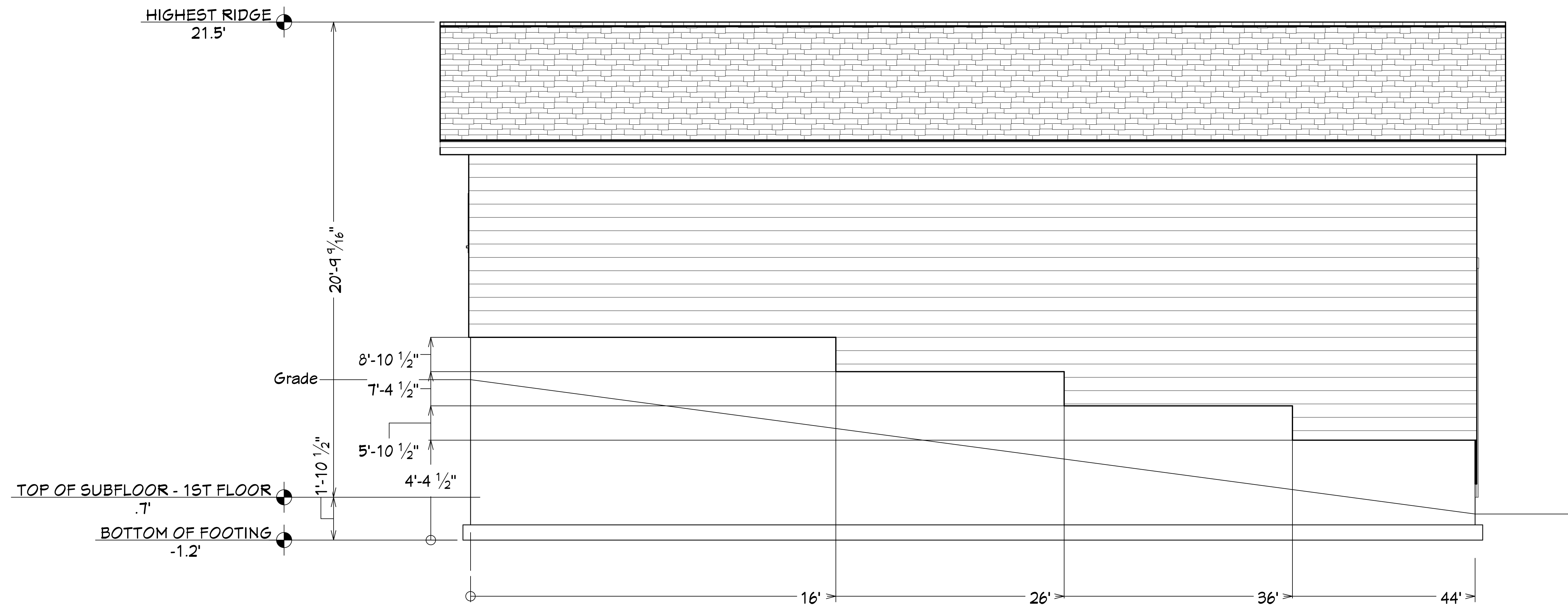
E8 EXTERIOR ELEVATION LEFT 3/8 IN = 1 FT
