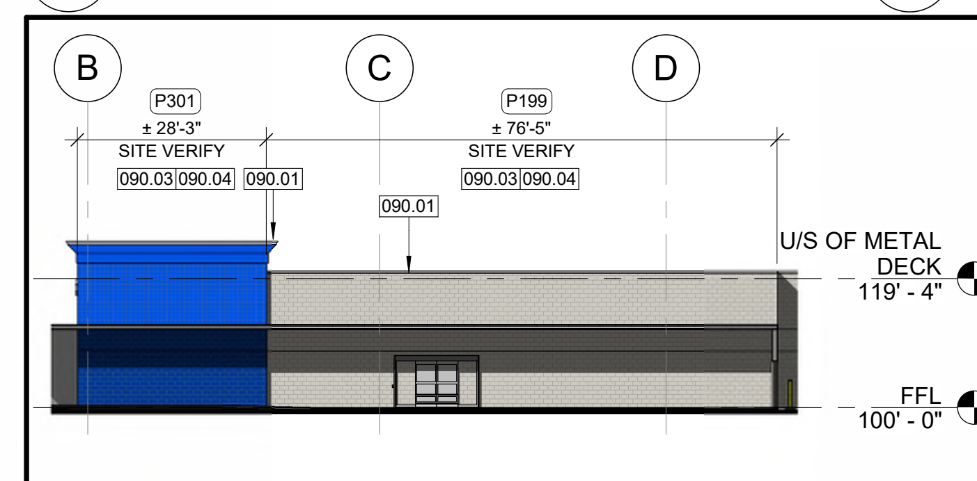
6 WEST (PARTIAL) ELEVATION I A2.0 1" = 20'-0"
