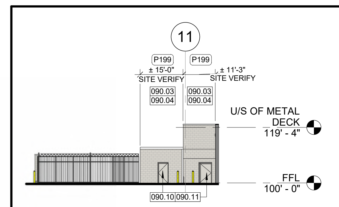
9 SOUTH (PARTIAL) ELEVATION A2.0 1" = 20'-0"
