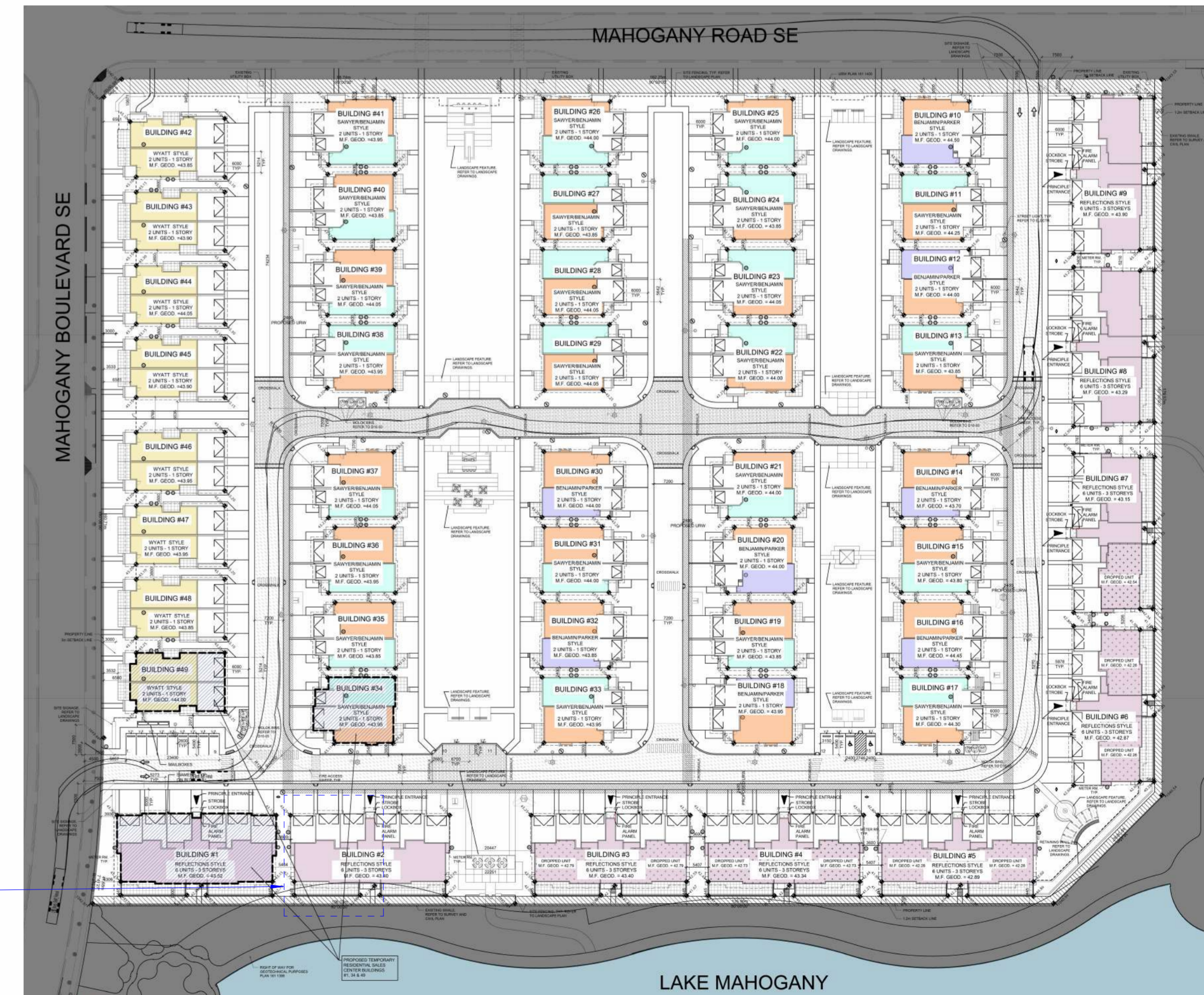
1 Site (Overall) 1: 1000
