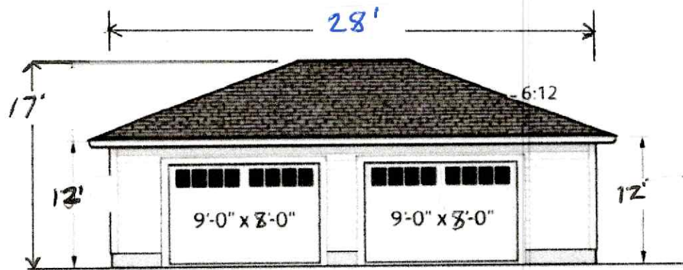
REAR ELEVATION
