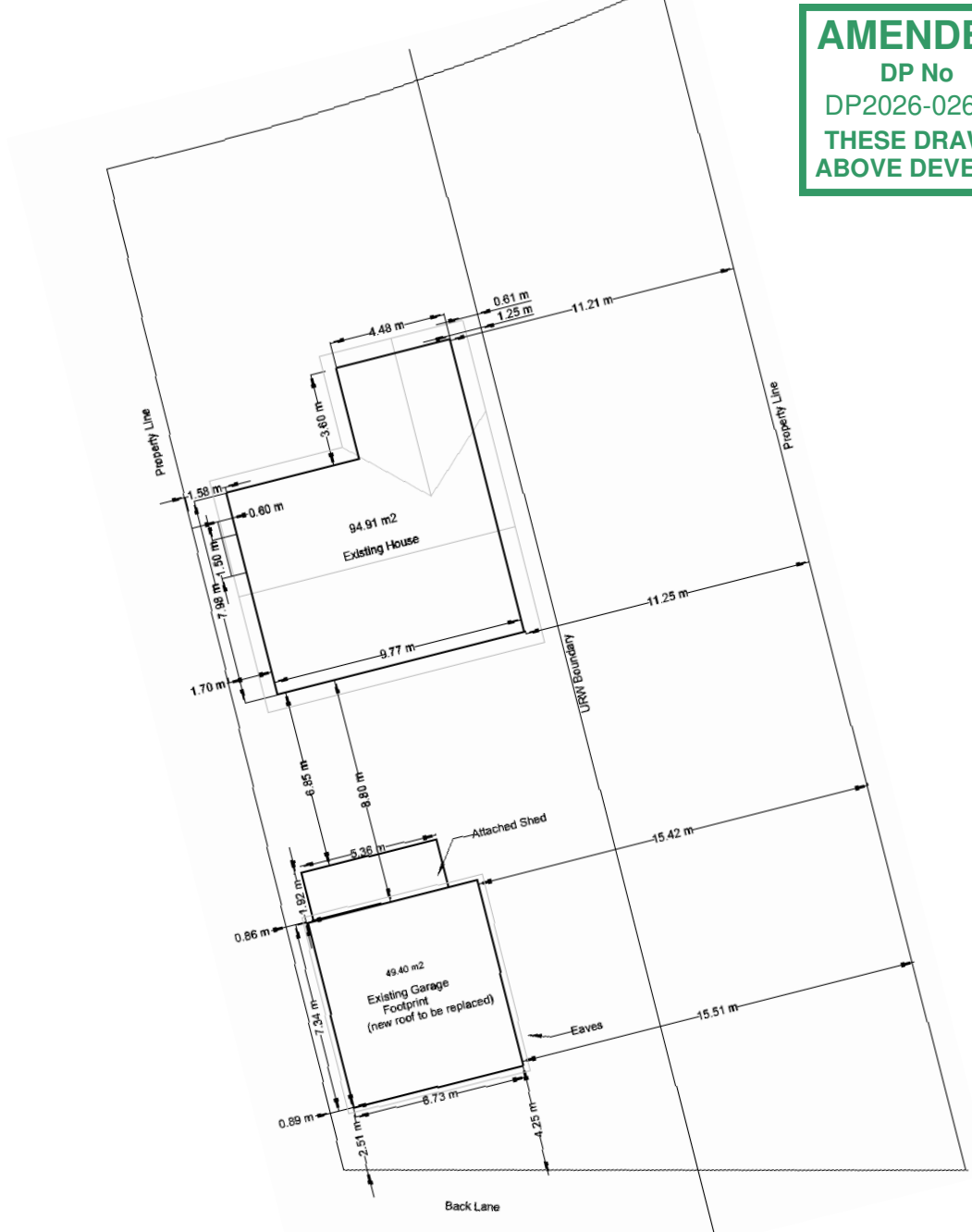
Existing Building Dimensions and Locations
