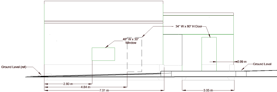
East Elevation
