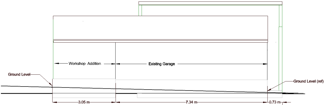
West Elevation
