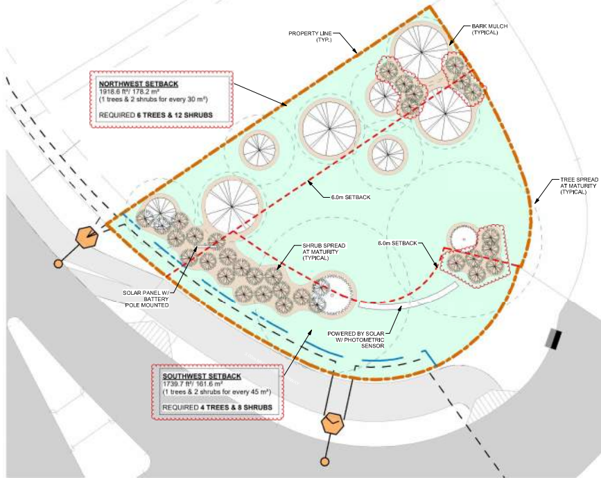
1 LANDSCAPING PLAN SCALE: 1:125
