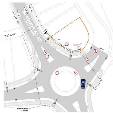
3 PHOTO TAG PLAN SCALE: 1:500
