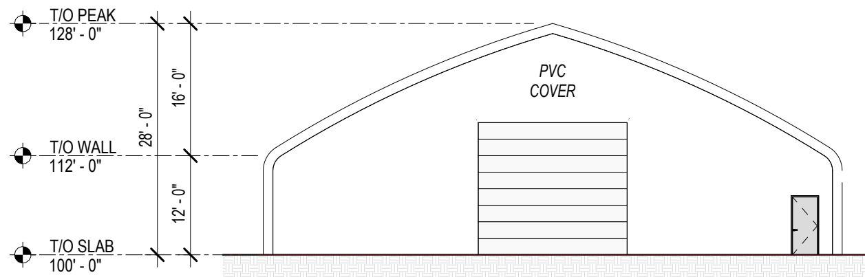
① WEST ELEVATION 1/16" = 1'-0"
