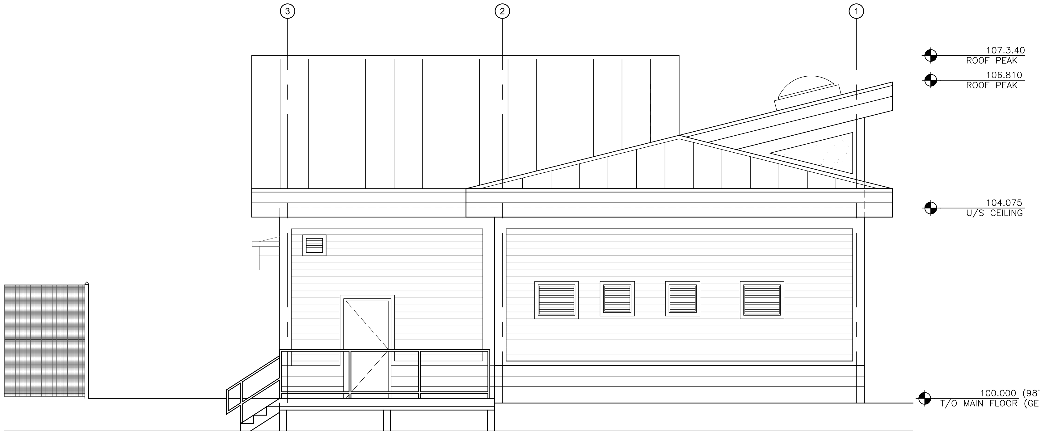
1 ELEVATION — REAR (NORTH) A3.2 SCALE: 1 : 50 P:\2402 URBAN SETON\DRAWINGS\2402-A-EL01.dwg
